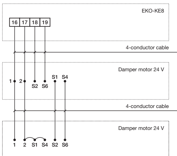
Damper group 1
