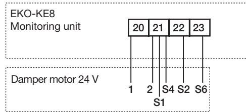
Damper 2
