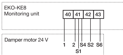
Damper 7
