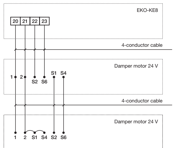
Damper group 2-4
