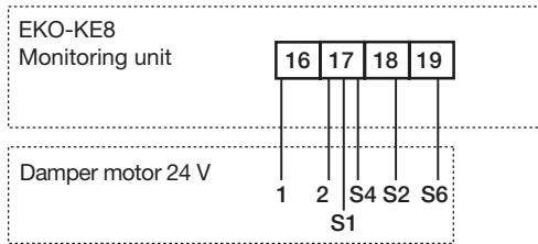
Damper 1
