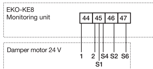
Damper 8
