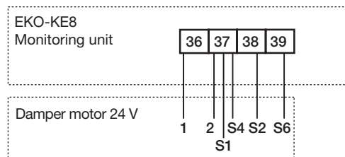
Damper 6
