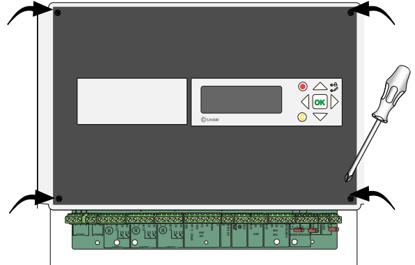
2. Unscrew and remove the front plate to access power supply, network cable and the rest of the circuit card.
